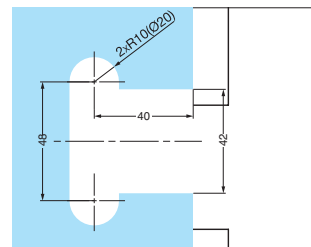
Bore Dimensions
