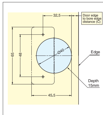
Bore Dimensions
